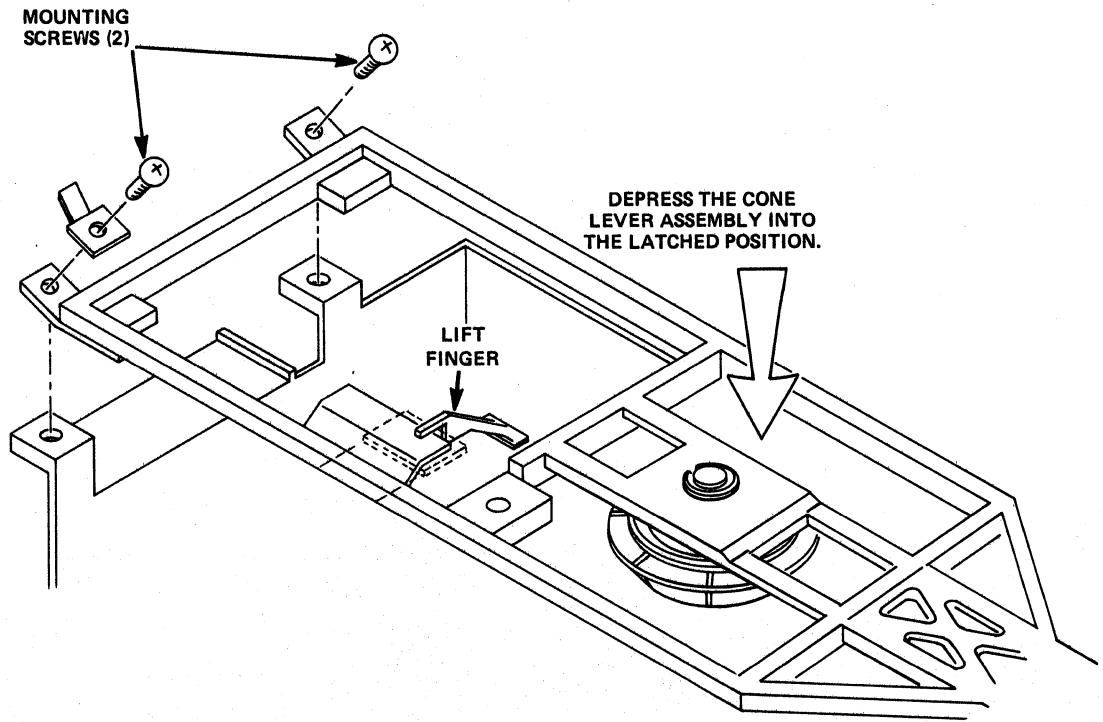
Figure 5-7 Cone Shaft and E-Ring
