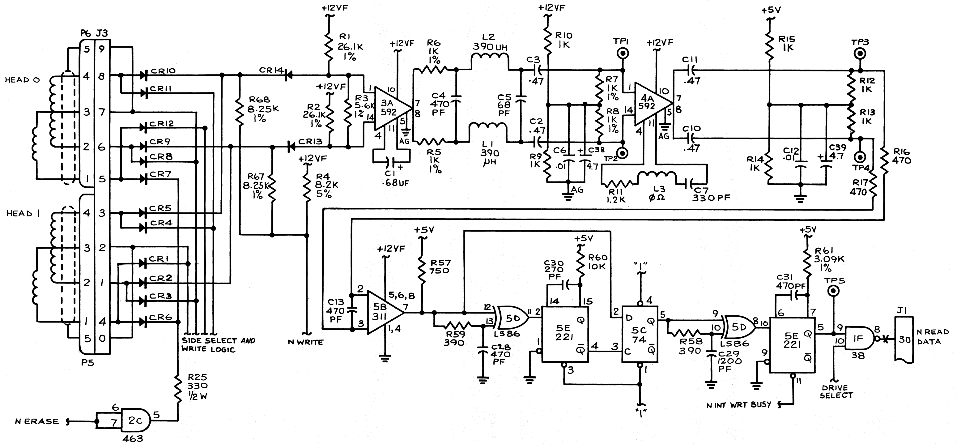
Figure 3-14 Read Data Schematic Diagram, Bipolar
