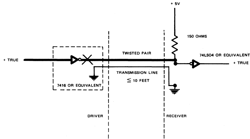
Figure 3-2 Interface Configuration
