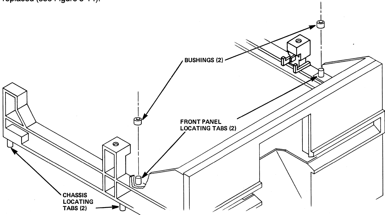
Figure 5-14 Front Panel Bushings, and Locating Tabs
