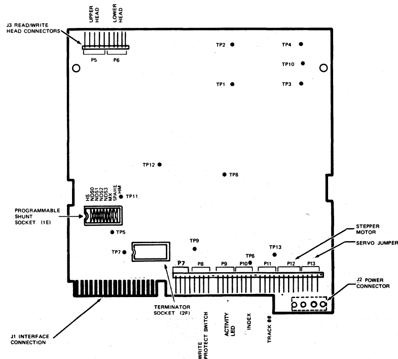
Figure 3-1 Logic PCBA
