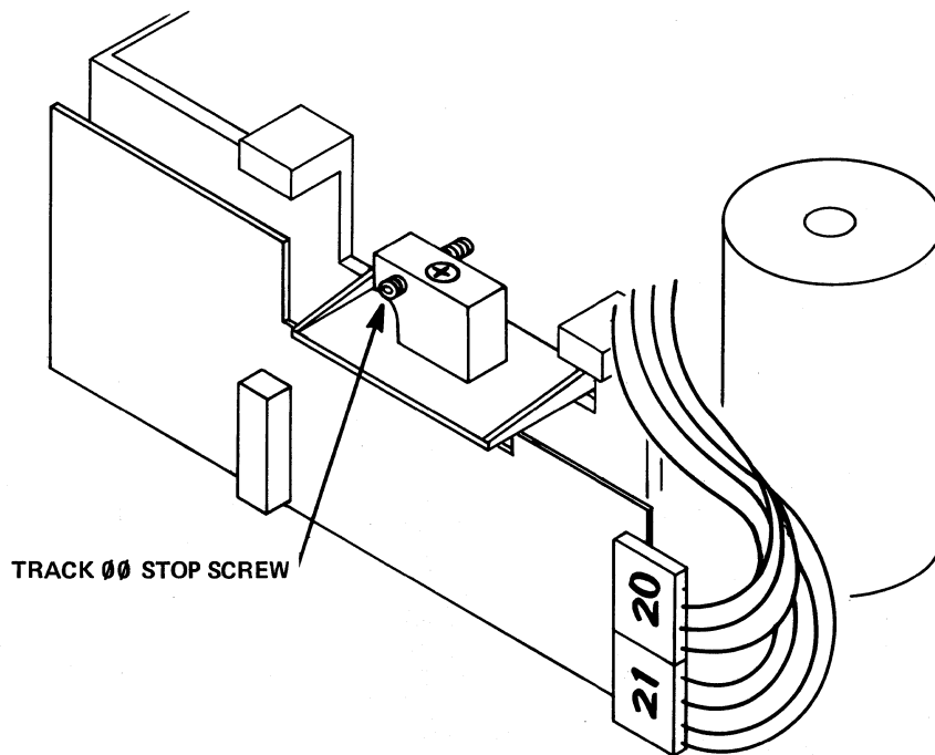
Figure 2-7 Track 00 Stop
