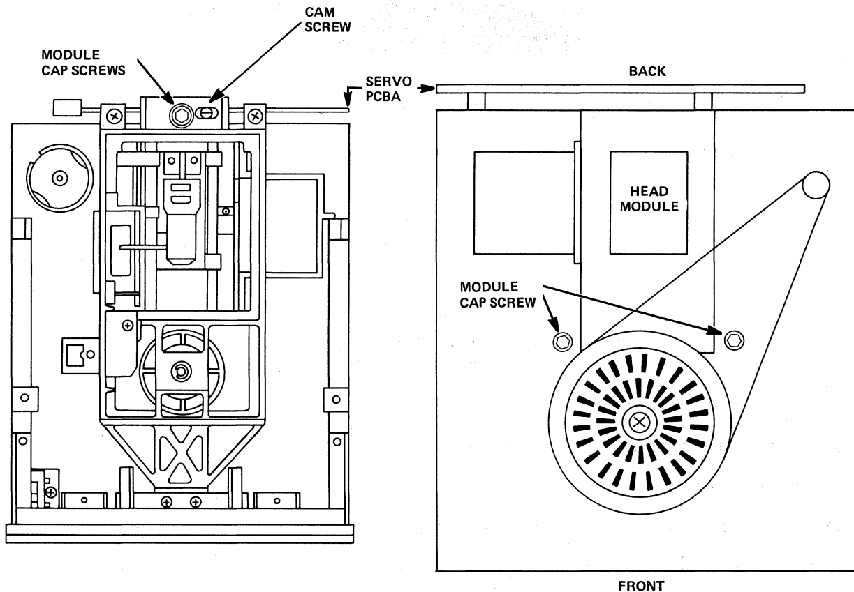
Figure 2-6 Head Module Cap and Cam Screws
