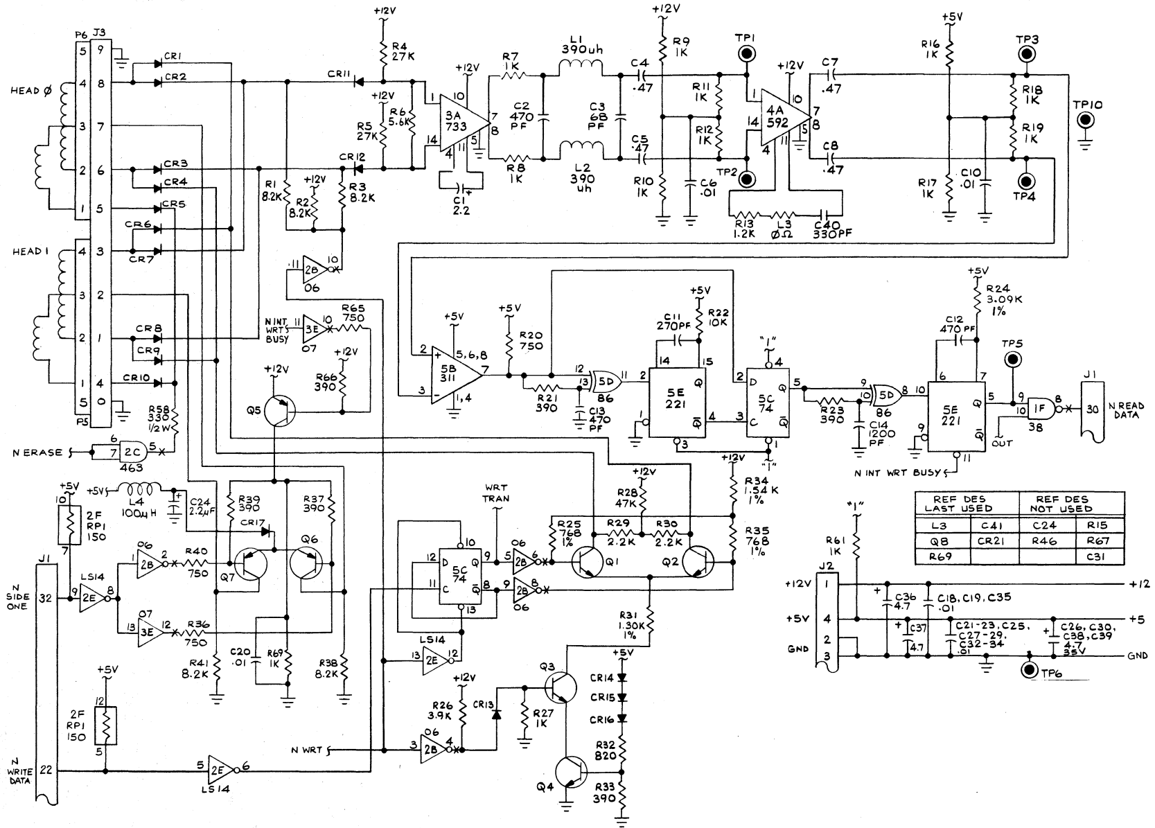
96/100 TPI, REWORK, UNIPOLAR LOGIC SCHEMATIC
